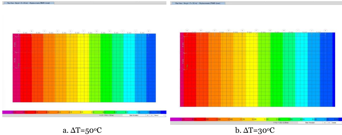
Fig. 4 Displacement result for building 24x50m without expansion joint
