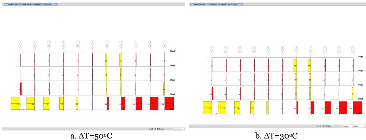
Fig. 9 Shear force result for building 24x50m without expansion joint
