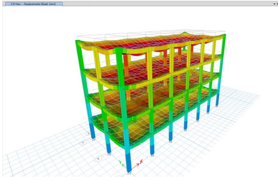
Fig. 2 3D ETABS model
