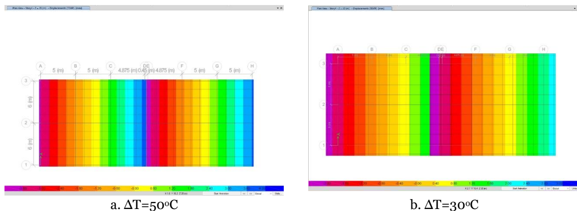
Fig. 5 Displacement result for building 12x30m with expansion joint
