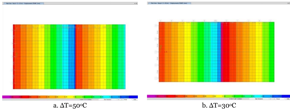
Fig. 3 Displacement result for building 24x50m with expansion joint
