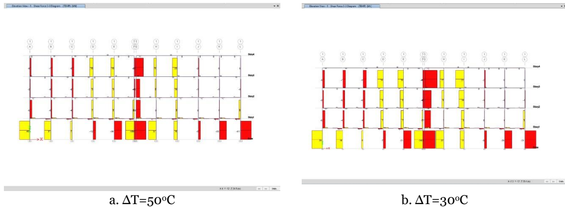
Fig. 8 Shear force result for building 24x50m with expansion joint
