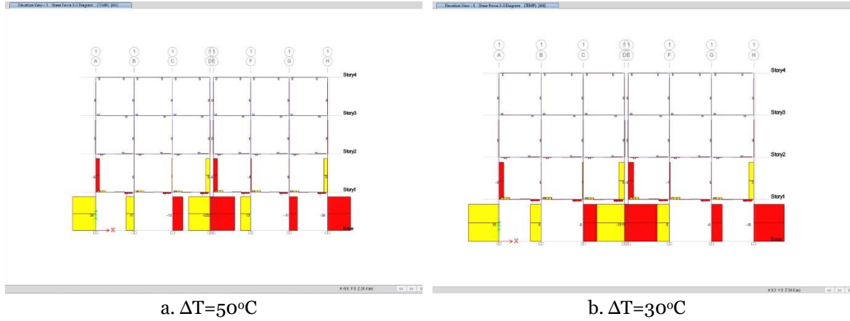
Fig. 10 Shear force result for building 12x30m with expansion joint
