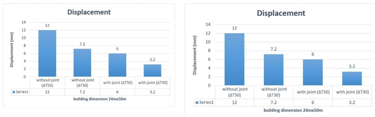
Fig. 7 Displacement result
