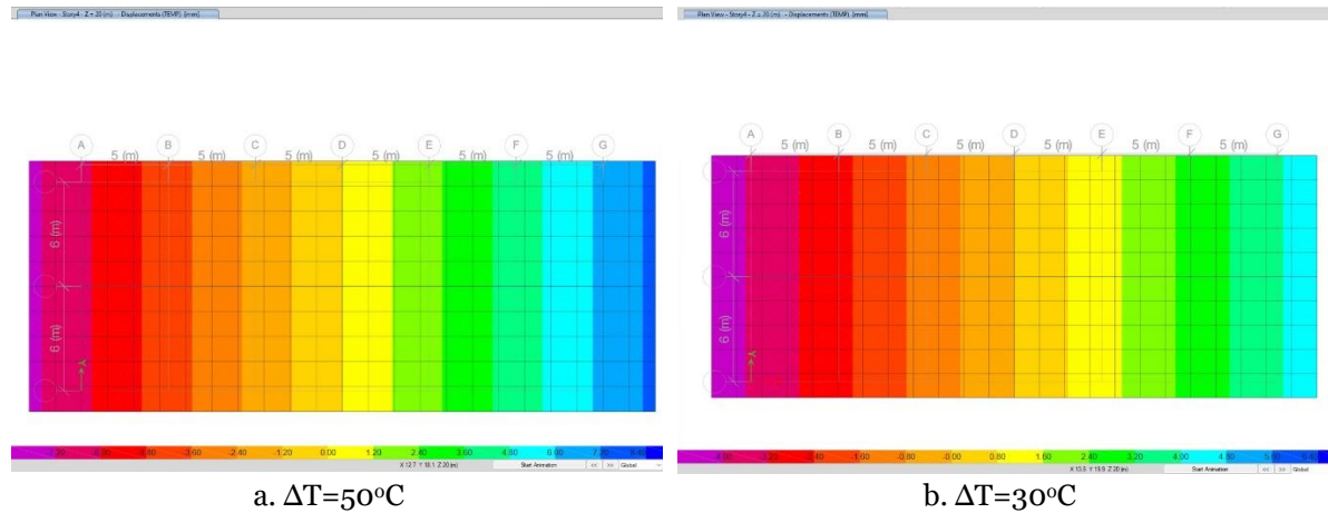
Fig. 6 Displacement result for building 12x30m without expansion joint
