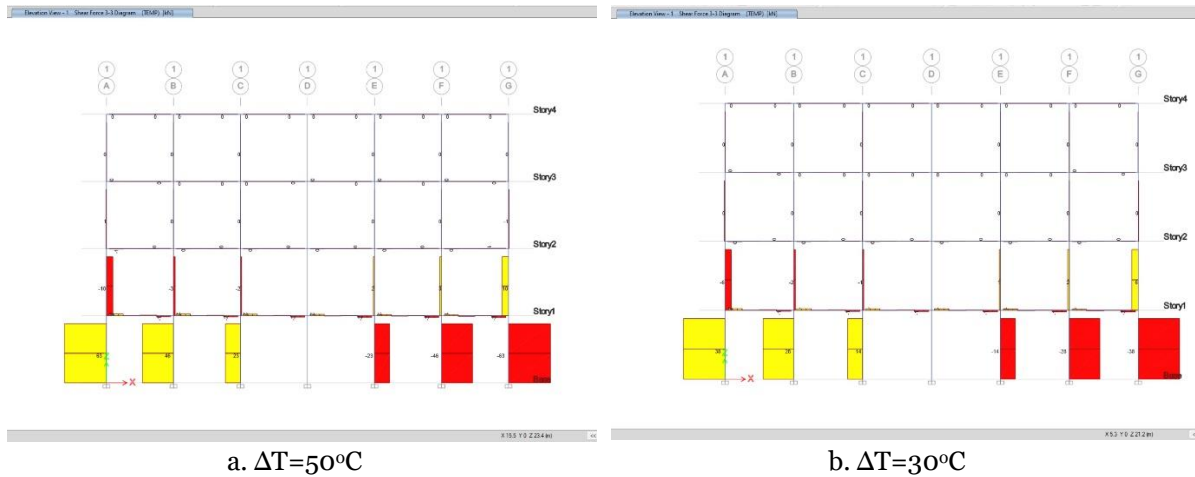
Fig. 11 Shear force result for building 12x30m without expansion joint
