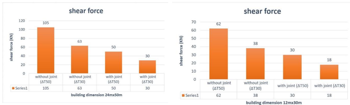
Fig. 12 Shear force result
